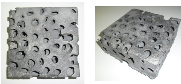
Fig. 6. Casting (cast iron with lamellar graphite) – type I
