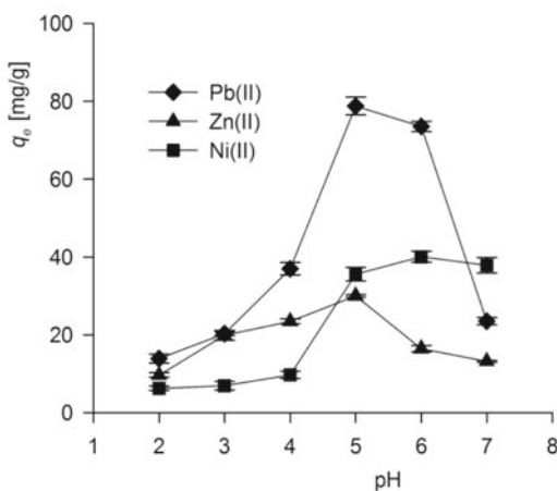
Figure 2. Effect of pH on the biosorption of Pb(II), Zn(II) and Ni(II) by Bacillus subtilis . Metal concentration: Pb(II) 98.4 mg/l, Zn(II) 39.6 mg/l, Ni(II) 45.6 mg/l, contact time 30 min
