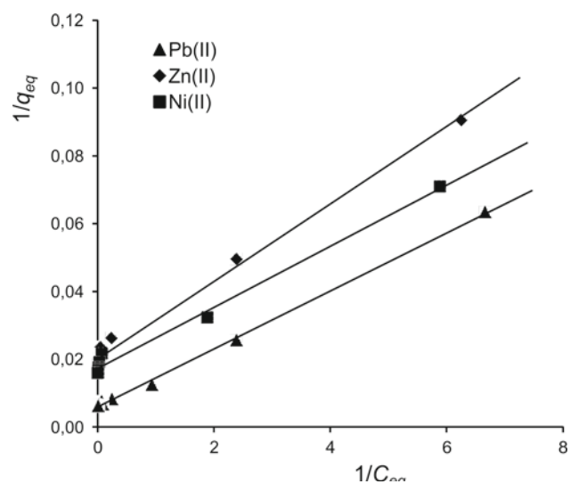
Figure 6. The linear from of Langmuir adsorption isotherm of Pb(II), Zn(II) and Ni(II) by Bacillus subtilis . Metal concentration: Pb(II) 15.9–325.3 mg/l, Zn(II) 11.2–172.3 mg/l, Ni(II) 14.3–245.8 mg/l, contact time 30 min., pH 5.5
