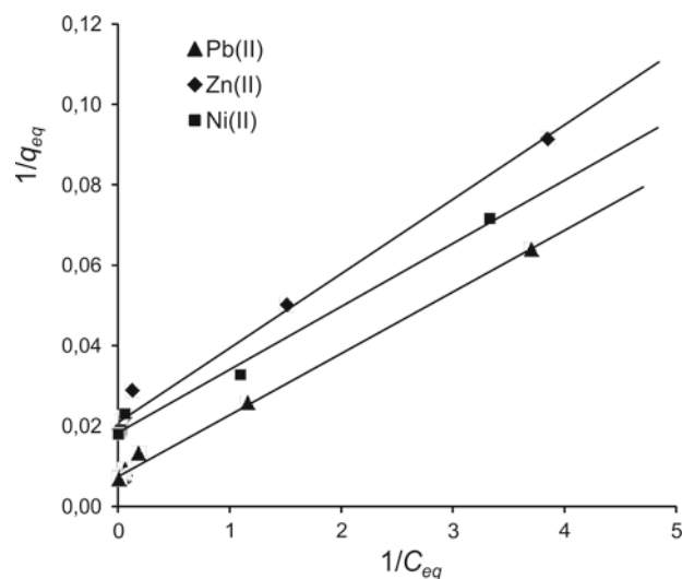
Figure 5. The linear from of Langmuir adsorption isotherm of Pb(II), Zn(II) and Ni(II) by Stenotrophomonas maltophilia . Metal concentration: Pb(II) 15.9–325.3 mg/l, Zn(II) 11.2–172.3 mg/l, Ni(II) 14.3–245.8 mg/l, contact time 30 min., pH 5.5
