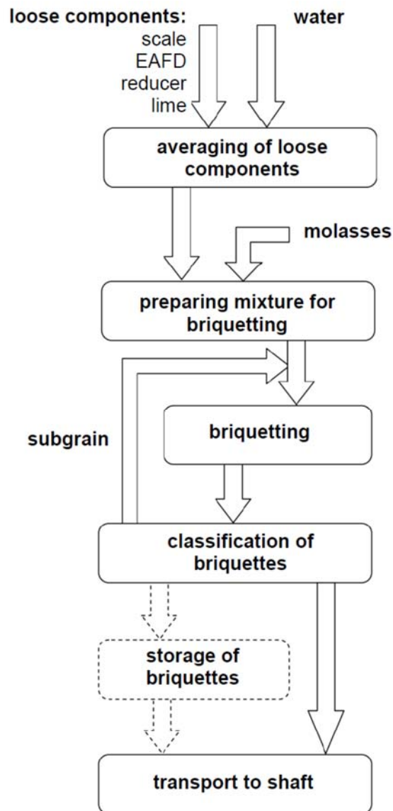
Fig. 5. A concept of briquetting mixtures containing a share of waste iron-bearing dusts containing zinc
