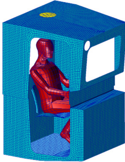
Fig. 8. Example of the calculation model of operator's cabins in the aspect of safety criterion
