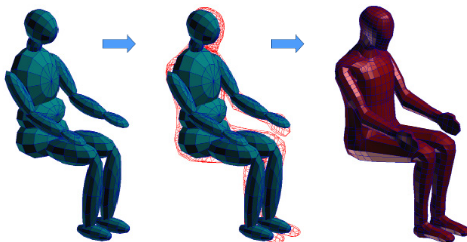
Fig. 5. Types of views computational model of Hybrid III dummy (Patran, 2012)
