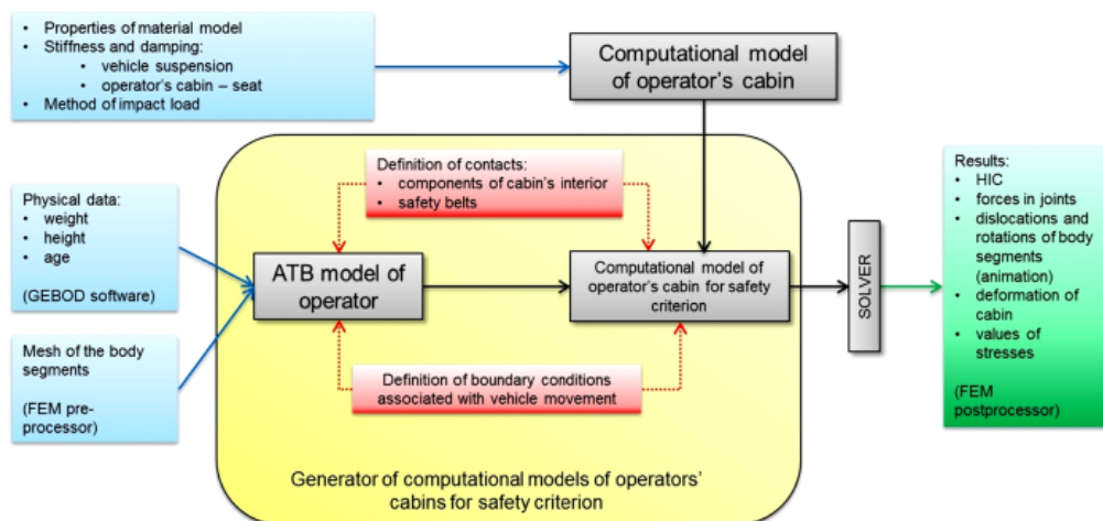
Fig. 6. Method of virtual prototyping of operators cabins in the aspect of safety criterion
