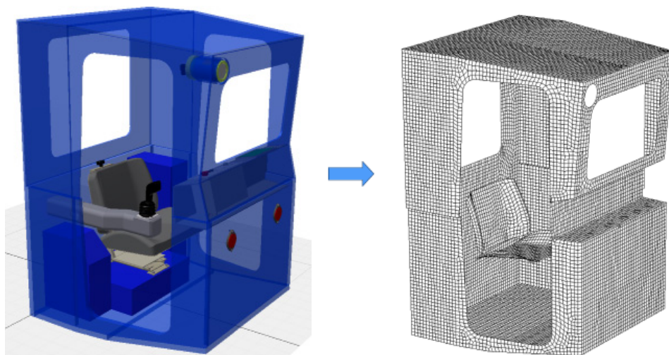
Fig. 7. 2D mesh of the calculation model of operator's cabin based on CAD model
