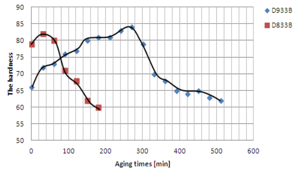
Fig. 8. Effect of the aging time pre-expanded raw materials on the patterns hardness
