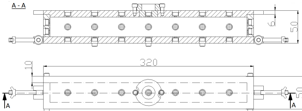
Fig. 3. Scheme of the matrix to prepare the samples for bending strength testing [7]
