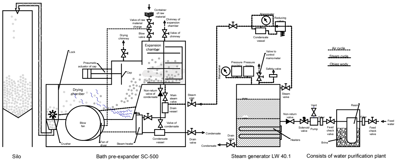
Fig. 1. Scheme station of polystyrene pre-expansion, equipped with a batch pre-expander [5]
