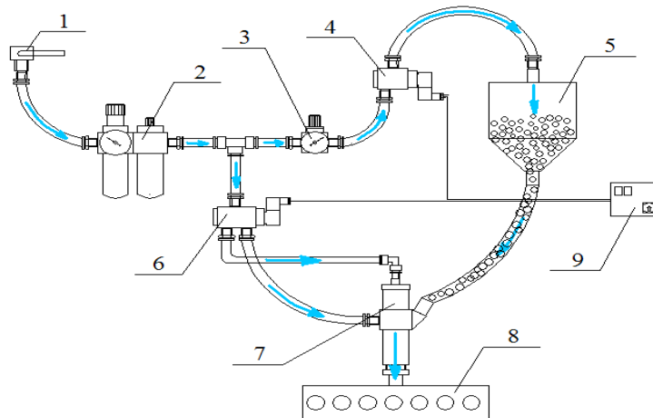
Fig. 4. The scheme of the workstation for filling the matrix with pre-expanded granules [7]
