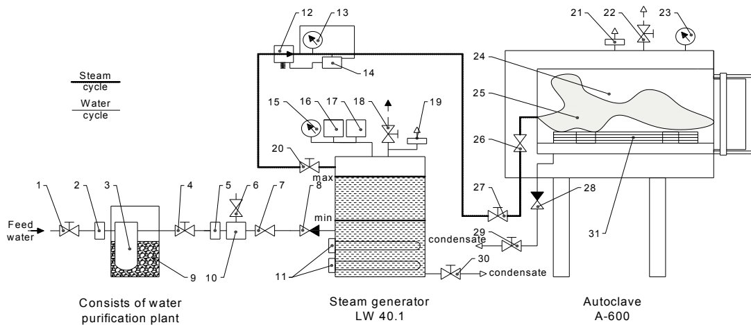
Fig. 2. Scheme of final forming position [6]
