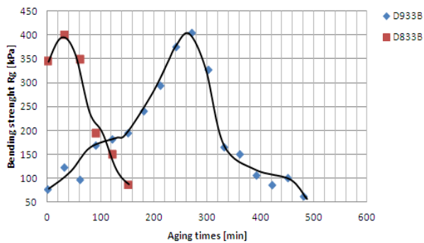
Fig. 7. Effect of aging time on the pre-expanded raw material for the bending strength polystyrene patterns
