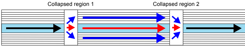
Fig. 1. The schematic of In-PCF MZI collapsing regions used to split and recombine the signals [13].
