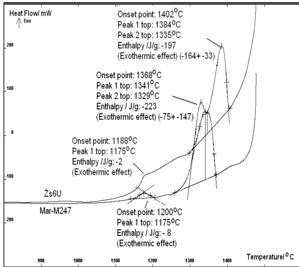
Fig. 2. Course of the DSC curve obtained during cooling for the Mar-M247 and Zs6U alloys
