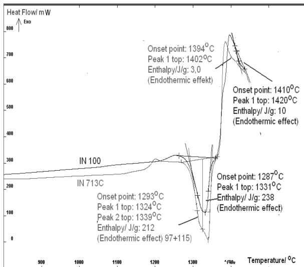
Fig. 3. Course of the DSC curve obtained during heating of the IN 100 and IN 713C alloys
