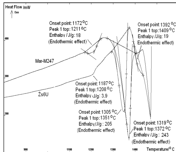
Fig. 1. Course of the DSC curve obtained during heating of the Mar-M247 and ŻS6U alloys
