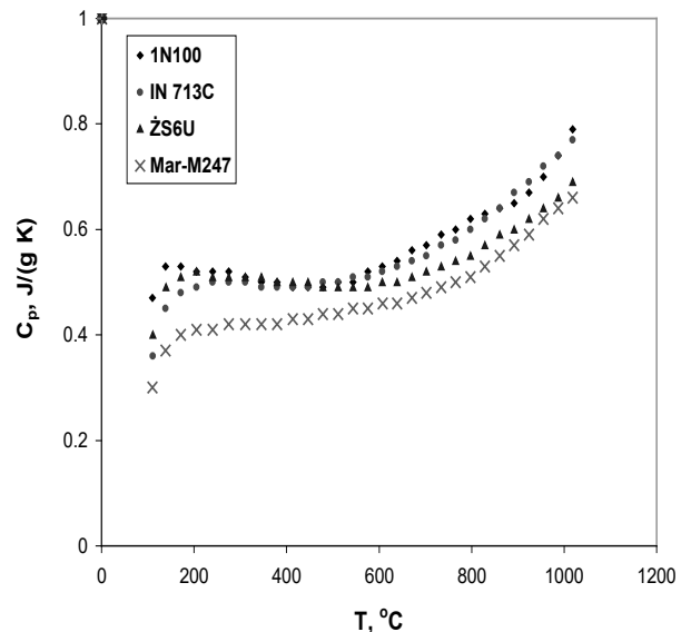
Fig. 5. The specific heat capacity of nickel superalloys vs. temperature
