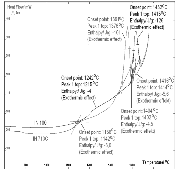
Fig. 4. Course of the DSC curve obtained during cooling of the IN 100 and IN 713C alloys
