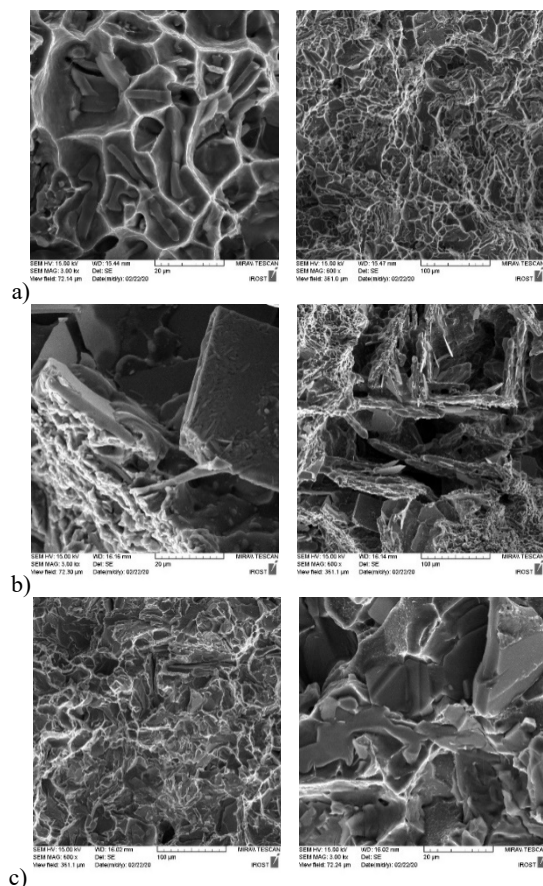
Fig. 8. The fracture surface of creep test at 275 °C and under (a) 75 MPa, (b) 125 MPa, and 150 MPa of the applied stress (Features included cleavage, guasi-cleavage, tear-ridge marks, micro-cracks and casting properties)
