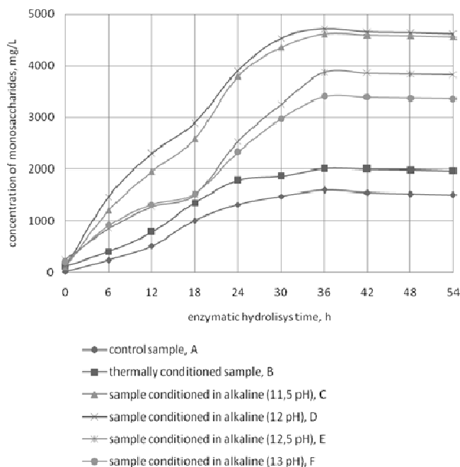
Fig. 1. Changes in the concentration of monosaccharides during enzymatic hydrolysis of homogenates
