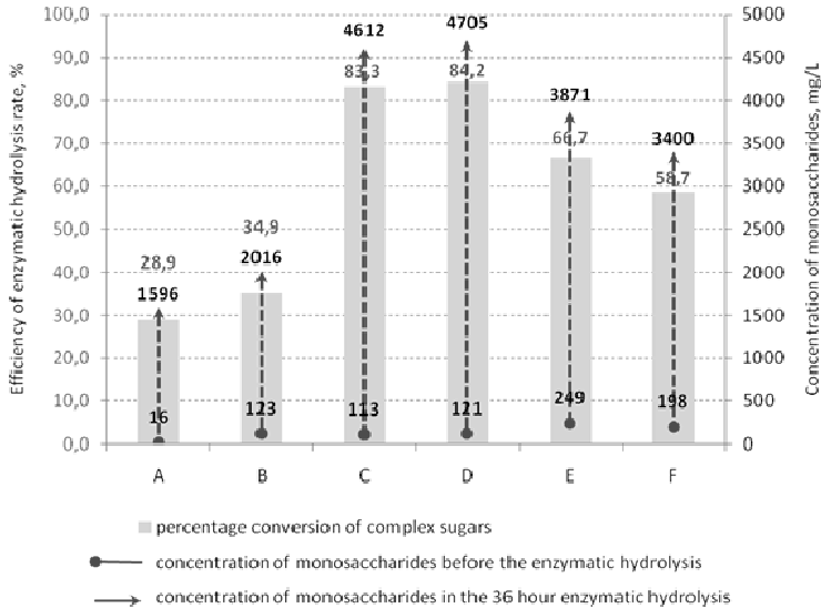
Fig. 2. The efficiency of the enzymatic hydrolysis and the increase in the concentration of monosaccharides during the 36 hours of the process – explanations are given in the text
