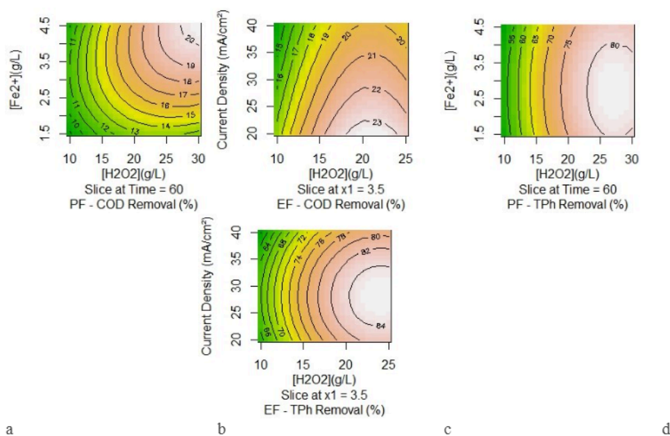
Fig. 3. Removal of COD and TPh from the effluent generated by the olive pomace oil extraction industry by PF and EF processes.
