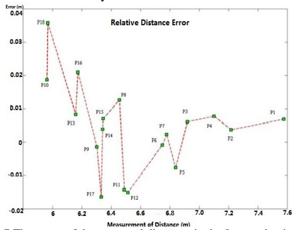
Fig. 7. The errors of the measured distances in the 9 control point case
