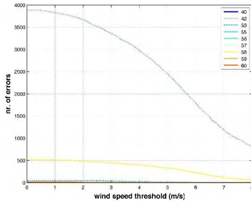
Fig. 6: Number of errors against wind intensity thresholds
