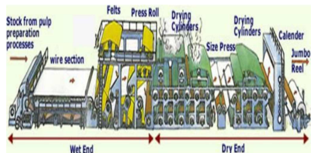
Fig. 2. Paper machine [18].
