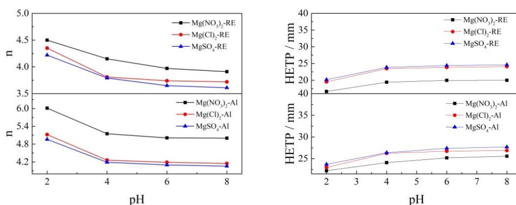
Fig. 7. Theory plate number curves of RE and Al; HETP of RE and Al under different pH
