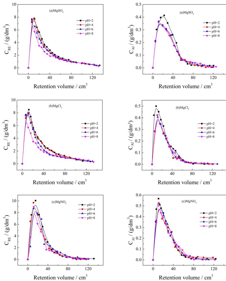
Fig. 6. Leaching behaviors of RE^{3+} and Al^{3+} (250 g of rare earth ore, C_{Mg^{2+}} = 0.2 \text{ mol/dm}^3 , \mu = 0.4 \text{ cm}^3/\text{min} , T=298\text{K} ): (a) MgSO_4 , (b) MgCl_2 , (c) Mg(NO_3)_2
