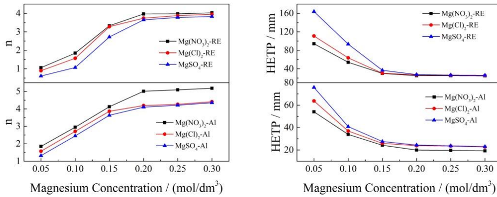
Fig. 5. Theory plate number curves of RE and Al; HETP of RE and Al under different magnesium concentration
