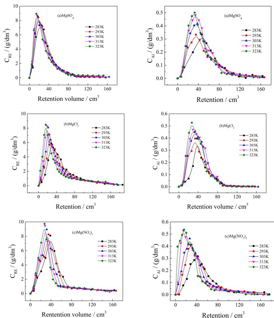
Fig. 8. Leaching behaviors of RE 3+ and Al 3+ (250 g of rare earth ore, C Mg2+ = 0.2 mol/dm 3 , μ = 0.4 cm 3 /min): (a) MgSO 4 , (b) MgCl 2 , (c) Mg(NO 3 ) 2
