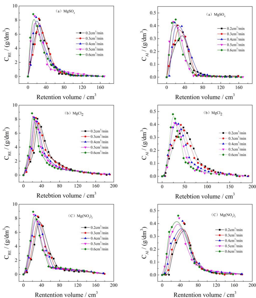
Fig. 2. Leaching behaviour of RE^{3+} and Al^{3+} (250 g of rare earth ore, C_{Mg^{2+}} = 0.2 \text{ mol/dm}^3 , T = 298\text{K} ); (a) MgSO_4 , (b) MgCl_2 , (c) Mg(NO_3)_2
