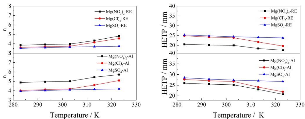
Fig. 9. Theory plate number curves of RE and Al; HETP of RE and Al under different temperature
