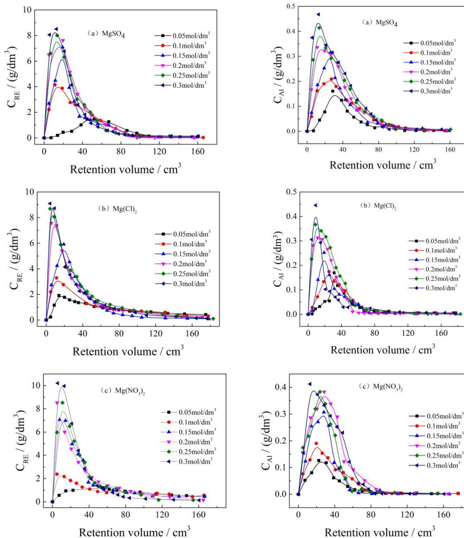
Fig. 4. Leaching behaviors of RE and Al (250 g of rare earth ore, \mu=0.4\text{cm}^3/\text{min} , T = 298\text{K} ): (a) \text{MgSO}_4 , (b) \text{MgCl}_2 , (c) \text{Mg}(\text{NO}_3)_2
