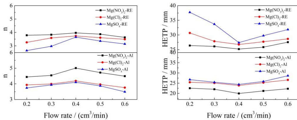
Fig. 3 Theory plate number curves of RE and Al; HETP of RE and Al under different flow rate
