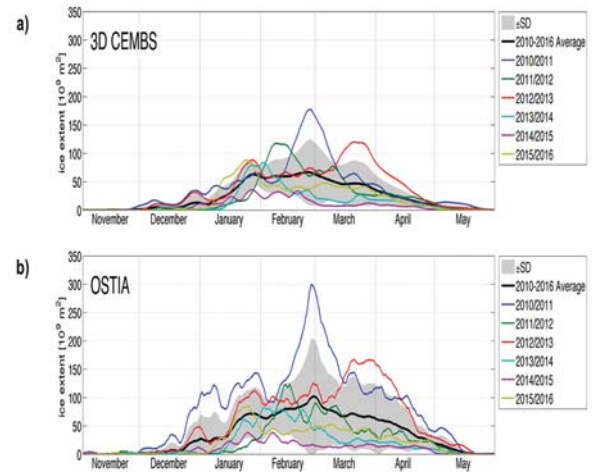
Fig. 3. Ice extent annual cycle for 3D CEMBS (a) and OSTIA (b). The black solid curve denotes the mean time evolution of ice extent area for the period 2010/2011–2015/2016 and the shaded area shows the range of variability defined by one added or subtracted standard deviation. 5-day trailing mean has been used
