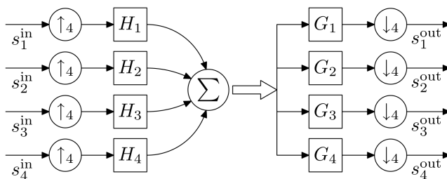
Figure 1: Transmultiplexer system
