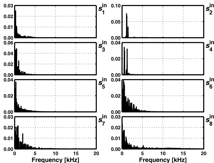
Figure 4: Amplitude spectra of the transmitted audio signals; the first is of speech and the others are of music
