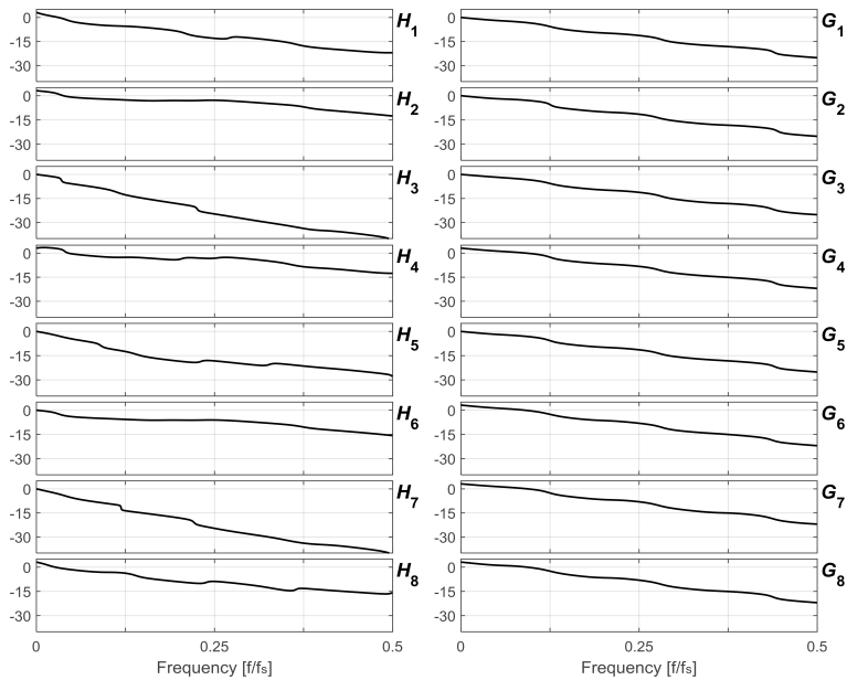
Figure 3: Phase characteristics of composition filters (left) and separation filters (right)
