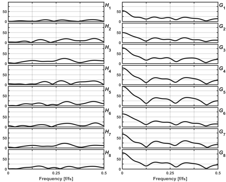
Figure 2: Amplitude characteristics of composition filters (left) and separation filters (right) for the case presented in Example 2, where f_s is a sampling frequency equal to 44 100 Hz
