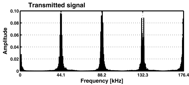
Figure 5: Spectrum of a signal obtained by transmultiplexing audio signals presented in Fig. 4
