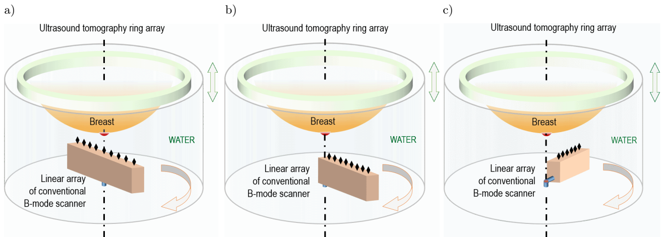
Fig. 3. Different multi-angle conventional ultrasound B-mode imaging (MACUI) methods designed as additional modality of developed prototype of ultrasound tomography scanner for in vivo female breast diagnosis, as an alternative to the FASCI method: a) with center of the additional linear array in the rotation axis, b) with edge of the additional linear array in the rotation axis, c) with edge of the additional linear array outside of the rotation axis.
