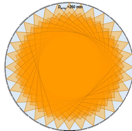
32 of 32-element ultrasonic subarrays of 1024-element ring array
