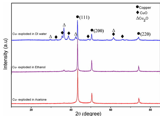
Fig. 1. XRD pattern of Cu nanopowder prepared by EEW in acetone, ethanol and DI water
