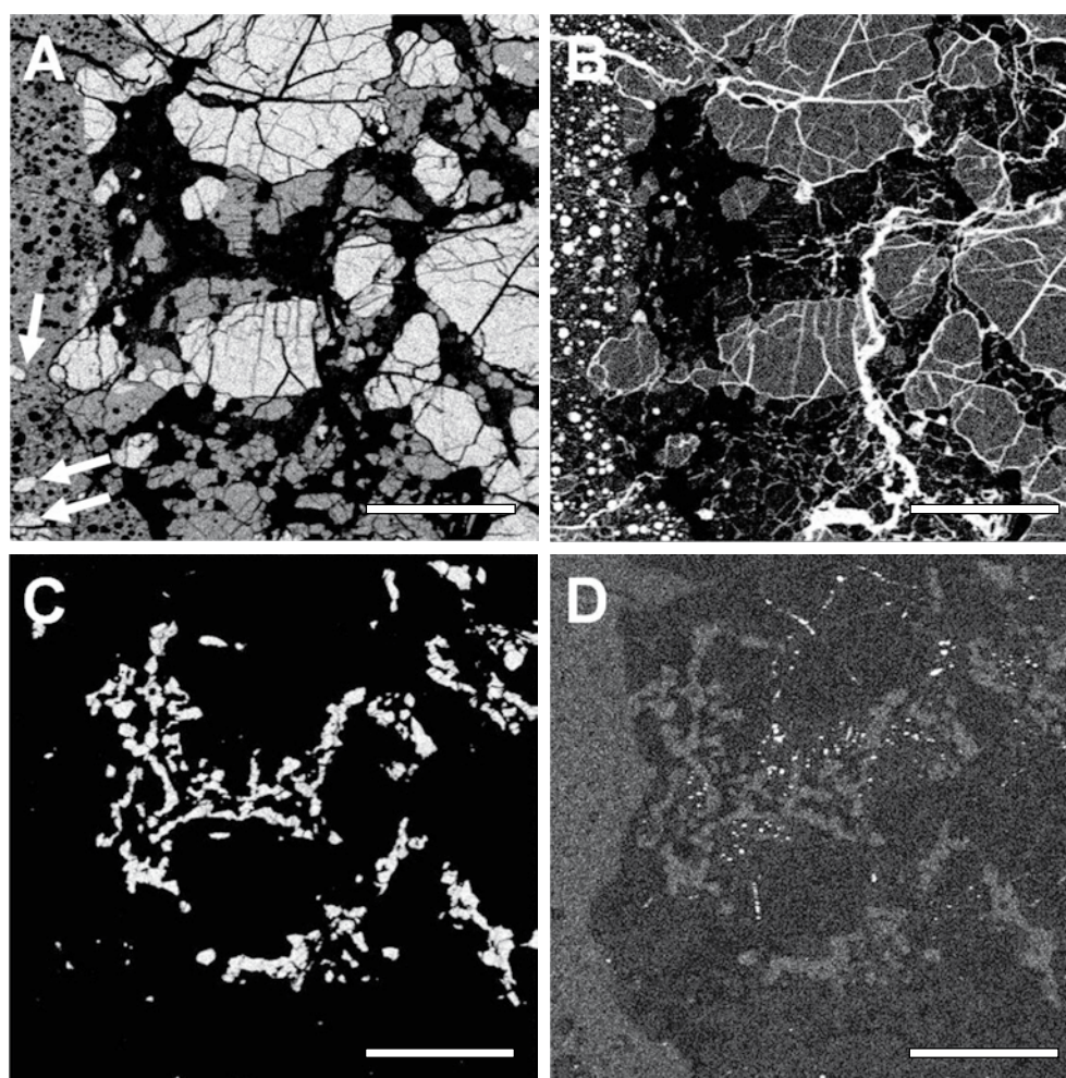
Fig. 3. Element map of the melts in Sahara 02500 (from upper left to lower right: Mg, Fe, Ca, Cr). Note the olivine phenocrysts (arrowed). Scale bars 100 \mu\text{m} .
