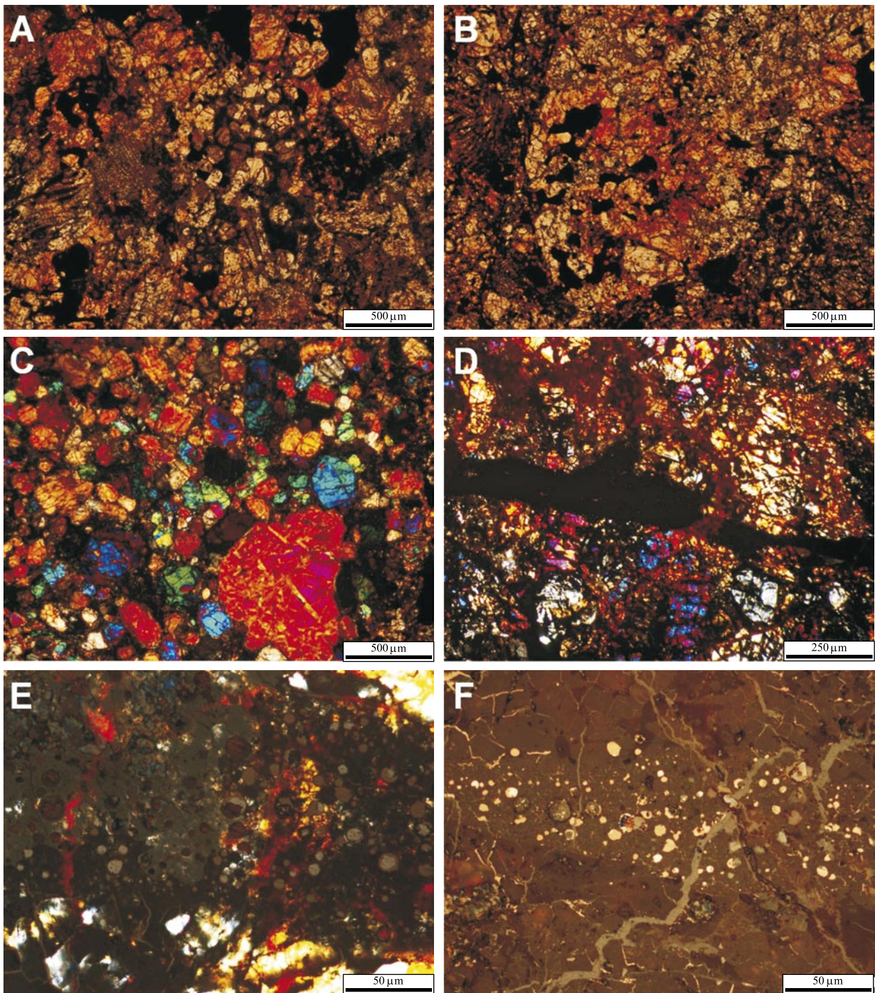
Fig. 1. Details of the Sahara 02500 meteorite (A-B and E transmitted light IIP, C-D transmitted light XP, F-reflected light IIP).
