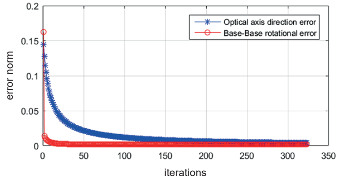
Fig.7. Recursive estimation of the base-base rotational error and optical axis direction error
