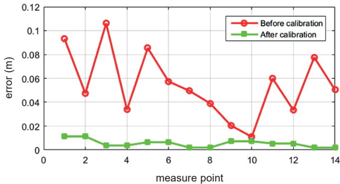
Fig. 8. Mismatch errors between optical axis vectors before and after calibration
