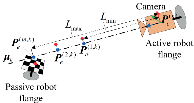
Fig. 3. Generated calibration poses of the passive robot corresponding to a calibration pose of the active robot
