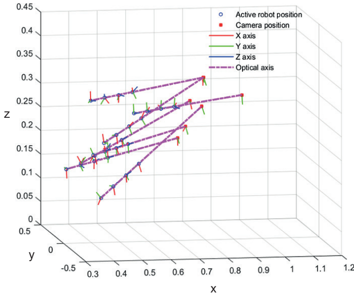
Fig. 6. The generated calibration poses of the two robots
