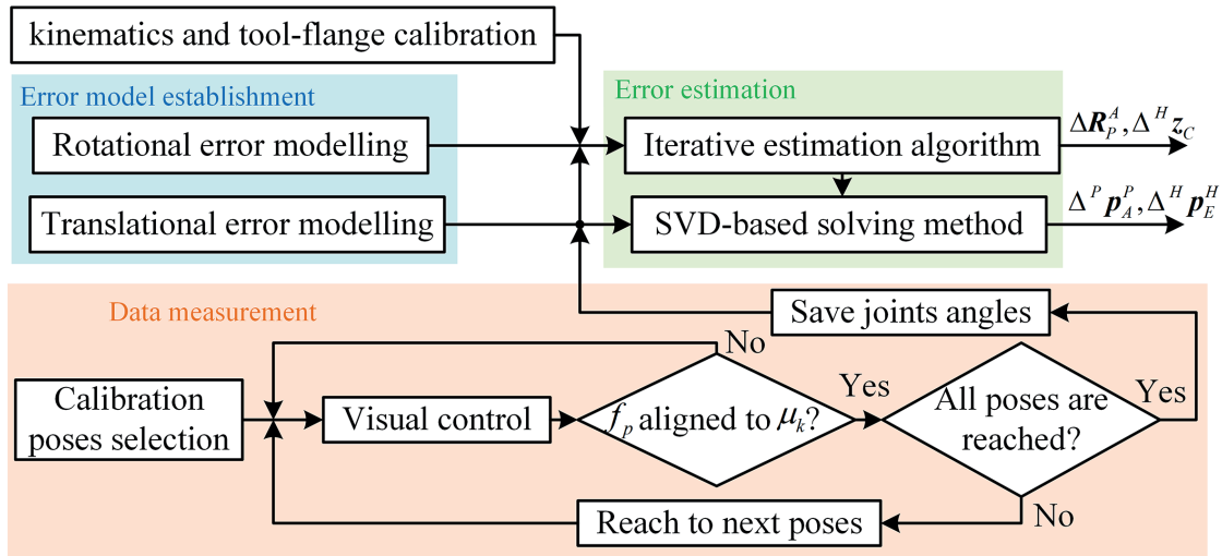
Fig.2. Scheme of the proposed calibration method
