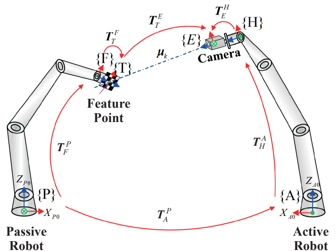
Fig. 1. Relative frames and transformation of the dual manipulator system
