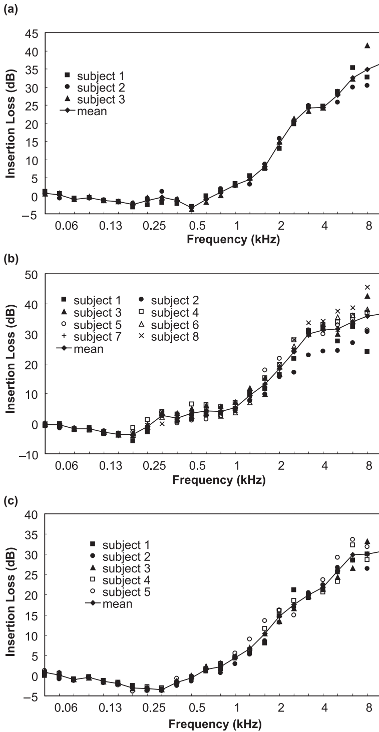
Figure 5. Insertion loss of Nolan (Italy) motorcycle helmets tested on subjects with MIRE (microphone in real ear); (a) Diamond N41 XL, (b) N102 XL, (c) N70 XL. Notes. Various symbols represent the spread of individual results. Solid line represents average insertion loss.
