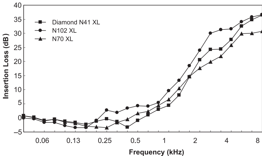
Figure 6. Insertion loss (mean values) of 3 Nolan (Italy) motorcycle helmets tested on subjects with MIRE (microphone in real ear).
