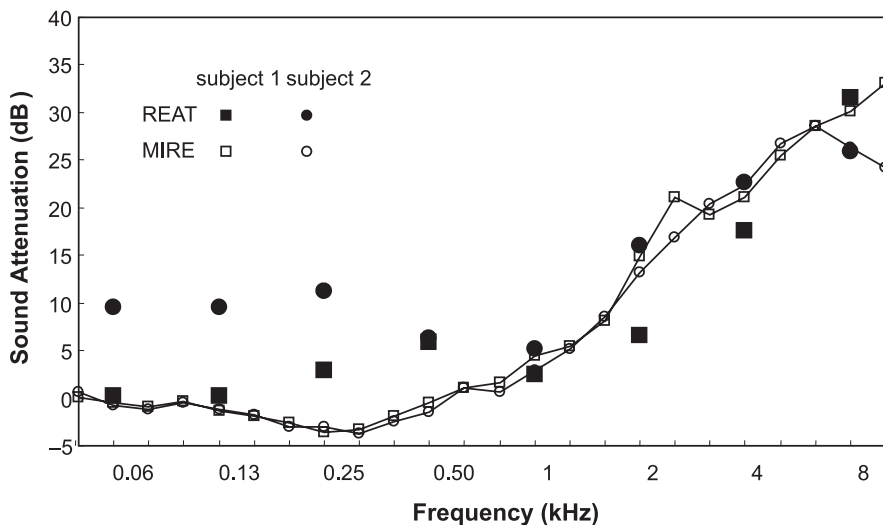
Figure 7. Sound attenuation measured on 2 subjects with REAT method (Nolan N70 XL). Notes. Solid lines show insertion loss measurements on the same subjects; REAT—real ear at threshold, MIRE—microphone in real ear.
