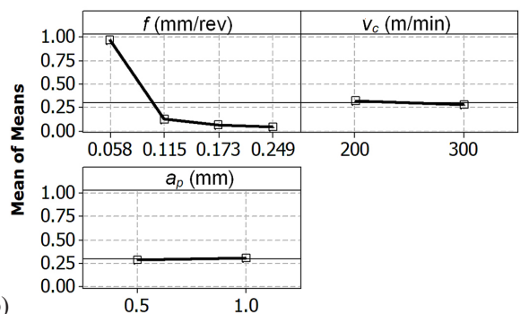
Fig. 3. Effect of test variables on the values of C_{in} . Turning of (a) laser sintered aluminum (b) cast aluminum
