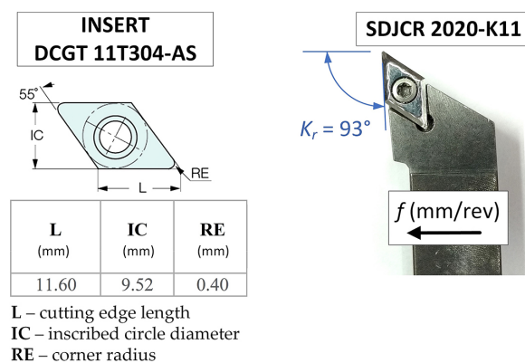
Fig. 2. The cutting tool
