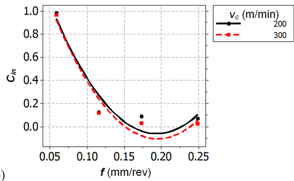
Fig. 4. C_{in} as a function of feed f . Turning of (a) laser sintered aluminum (b) cast aluminum
