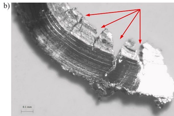
Fig. 5. Cracks on the inner (a) and outer (b) surface of the chip – turning of sintered material
