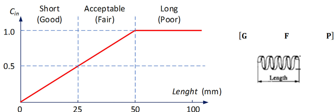
Fig. 1. Simplified classification of chip geometry (due to the length of chip ( L_{ch} )) [26]
