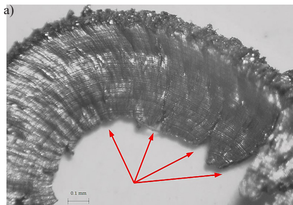
Fig. 5. Cracks on the inner (a) and outer (b) surface of the chip – turning of sintered material
