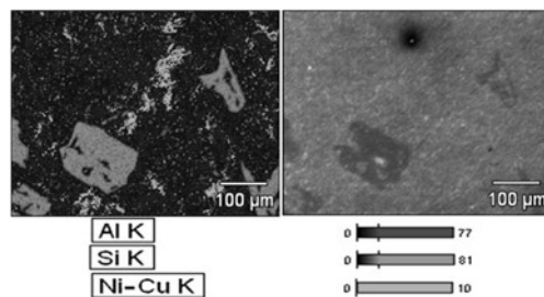
Fig. 2. Depiction of AlSi21CuNi surface from SEM microscope and a map of chemical elements distribution for this alloy
