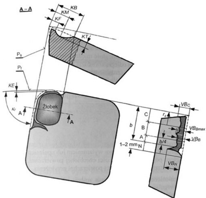
Fig. 1. Wear indices [1]
