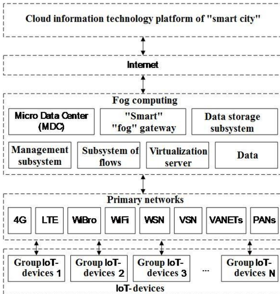
Fig. 1. Generalized architecture of "fog computing".
