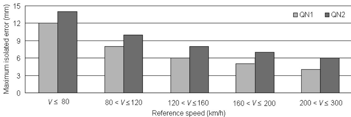
Fig. 4. The peak values for lateral alignment for track quality levels QN1 and QN2
