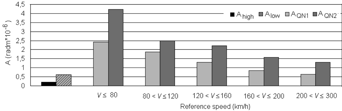
Fig. 5. The track quality coefficient
