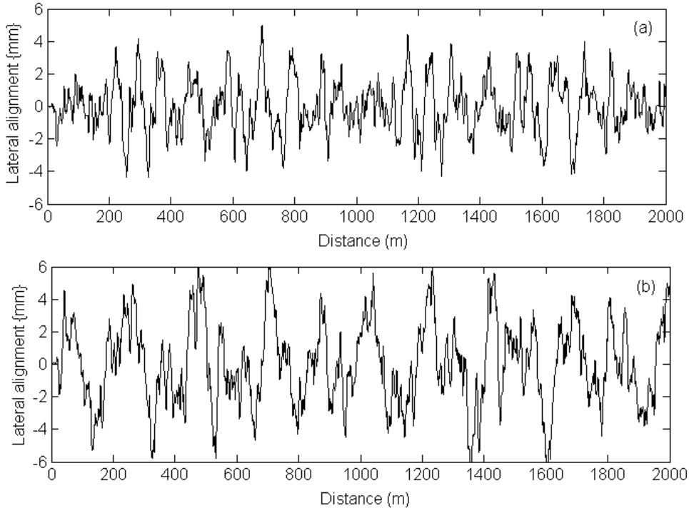
Fig. 7. The track alignment synthesis: (a) track quality level QN1; (b) track quality level QN2
