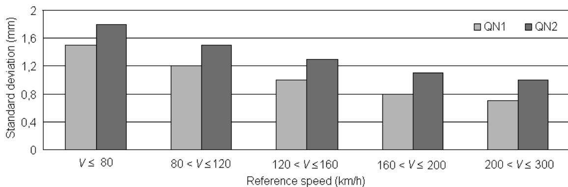
Fig. 3. Standard deviation for alignment for track quality levels QN1 and QN2
