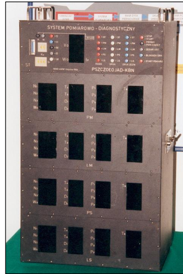
Fig. 15. Measuring and recording system 'PSZCZOŁOJAD' [15]
