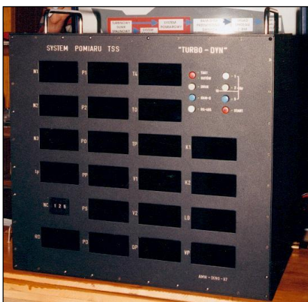
Fig. 16. Measuring and recording system 'TURBODYN' [15]
