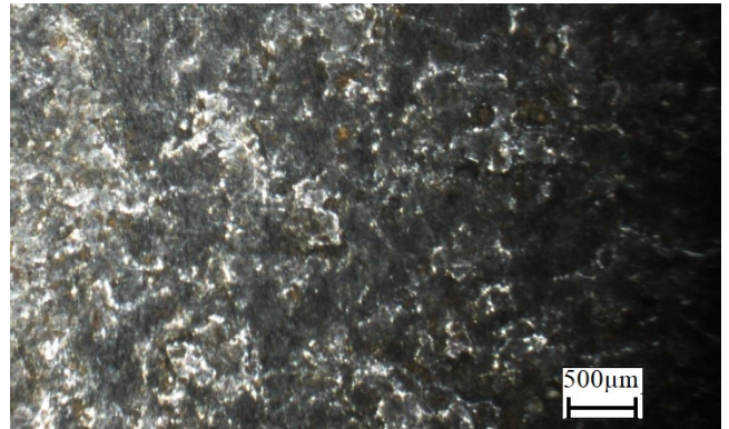
Fig.6. OM image of the surface before AWJ cutting. \times 10 .
