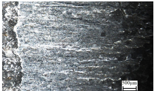
Fig.7. OM image of the surface after AWJ cutting, \times 10
