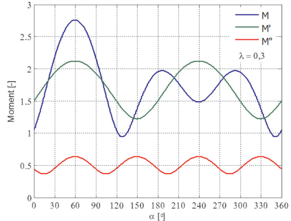
Fig. 4. Plots of the moment of the inertia forces \mathbf{M}' and \mathbf{M}'' and their sum \mathbf{M} in V6 engines with split-pin crankshafts, for \lambda = 0.3 , \gamma = 90^\circ and \delta = 30^\circ
