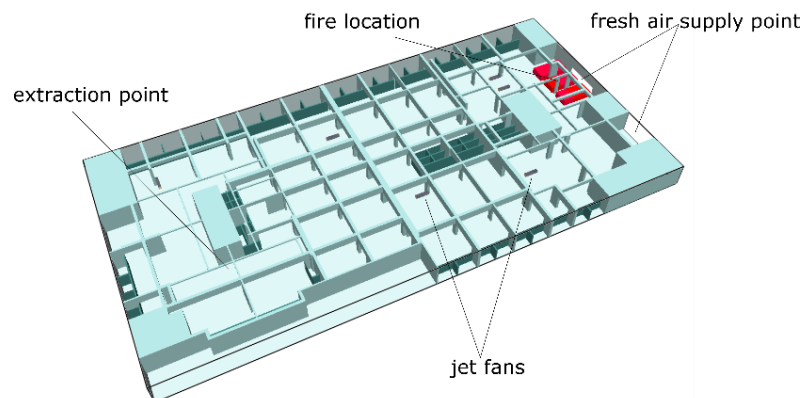
Figure 5. Three-dimensional model of the considered space
