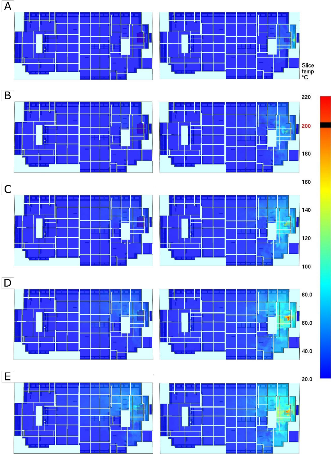
Figure 8. Results of temperature distribution at the height of 1.8 m above the floor for the model fire according to BS 7346-7:2013 standard (curve 1) on the left side and according to NEN 6098:2010 (curve 2) on the right side of the figure respectively for the times from fire initiation: A - 60 s, B - 120 s, C - 180 s, D - 240 s, E - 300 s.
