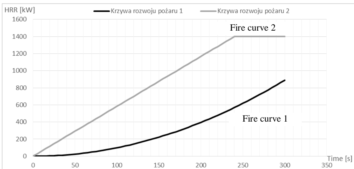
Figure 4. Course of fire development curves based on BS 7346-7:2013 standard, \alpha = 0.00988 \text{ kW/s}^2 , (curve 1) and according to NEN 6098:2010 (curve 2) during the evacuation time in the considered underground garage, own elaboration based on [11], [12].
