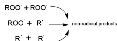
Fig. 1. Mechanism of free radical oxidation
