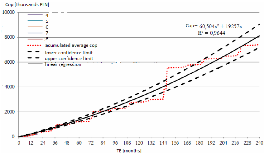
Figure 11. Preventive maintenance costs of rail buses of chosen type [9]
