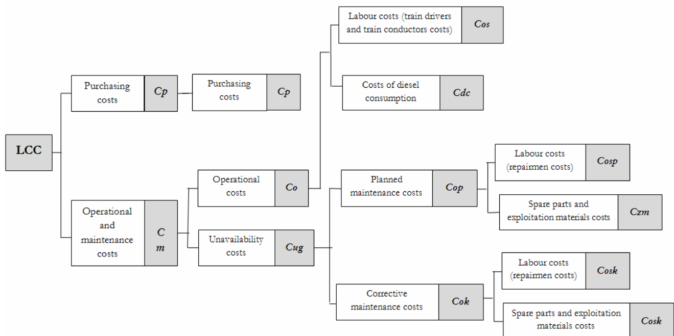
Figure 9. Cost structure used in LCC analysis of railcars [9].
