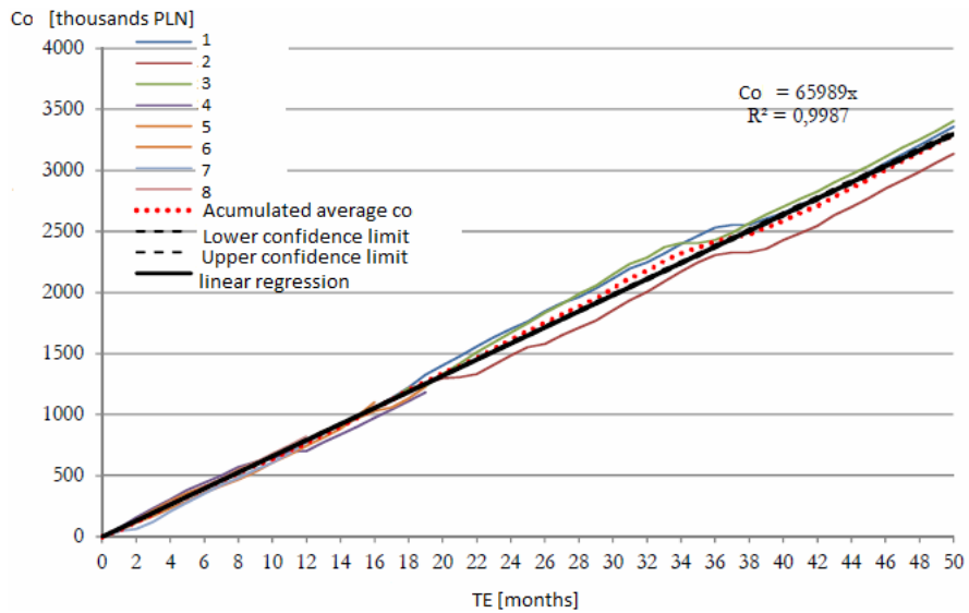
Figure 10. Operational costs of analysed rail buses [9]
