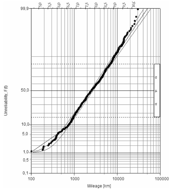
Figure 6. The cumulative distribution function of rail buses time between failures [mileage]
