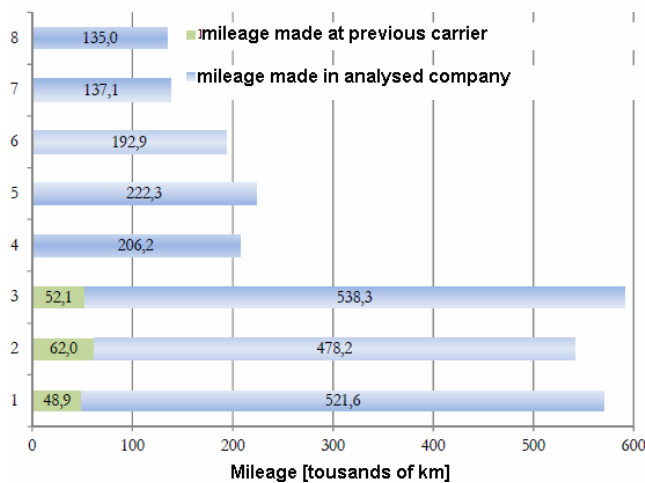
Figure 4. Working time of rail buses defined as a mileage [9]
