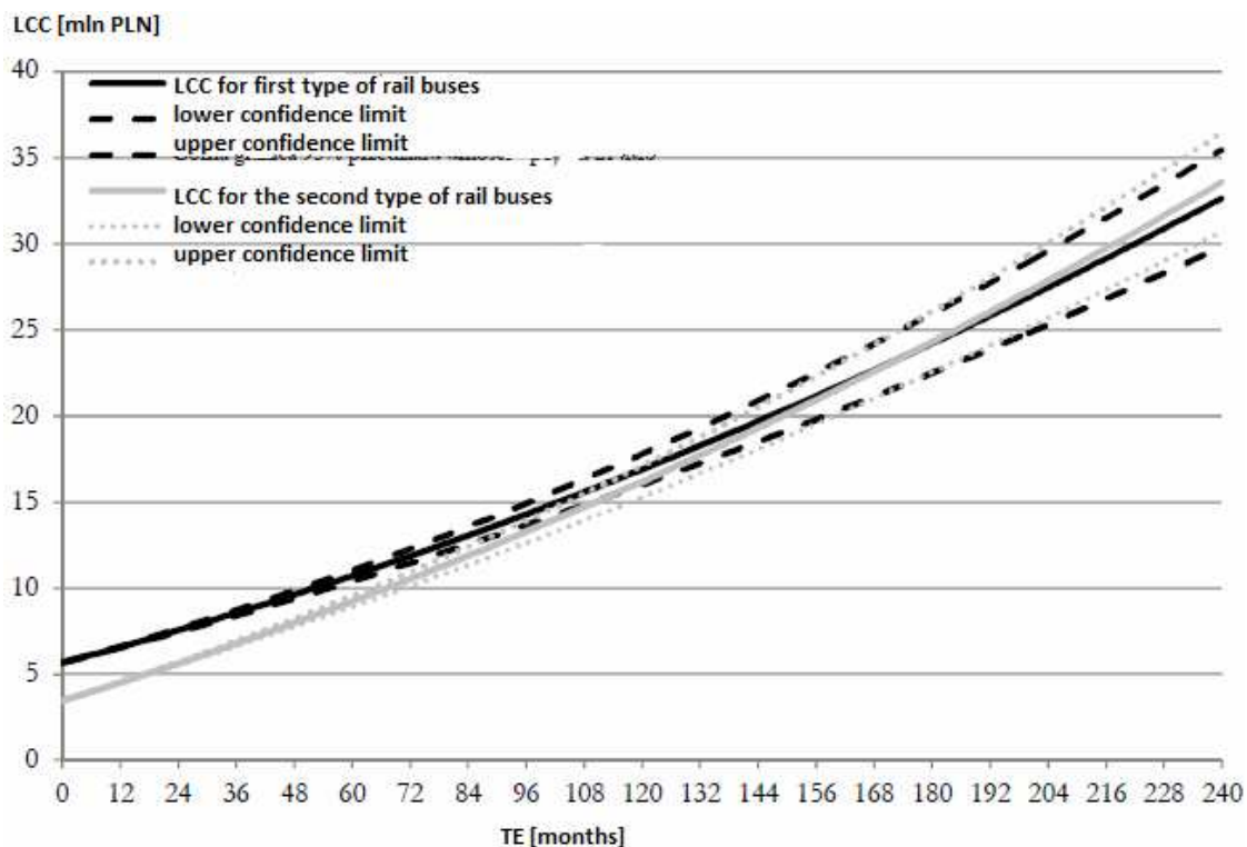
Figure 13. LCC for analysed types of rail buses [9]
