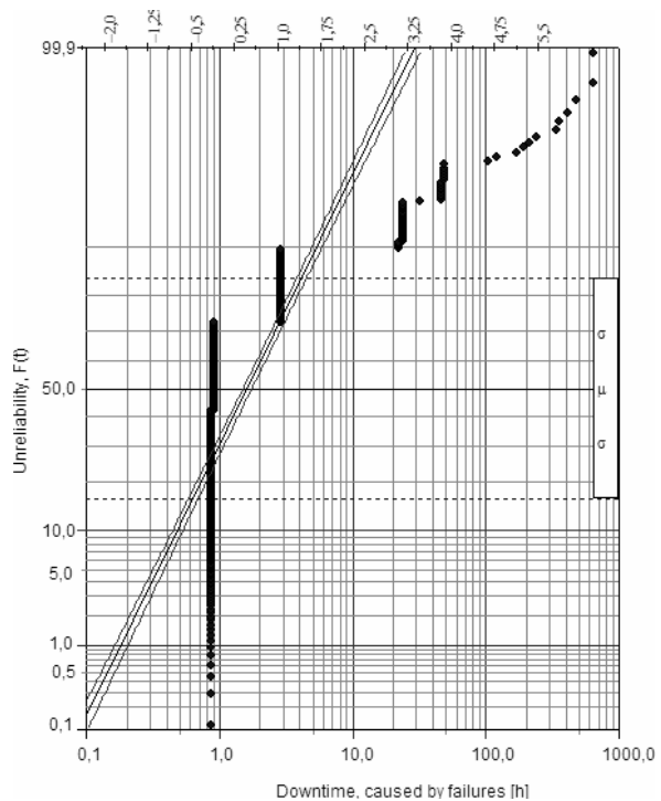
Figure 7. The cumulative distribution function of rail buses repair time [hours]
