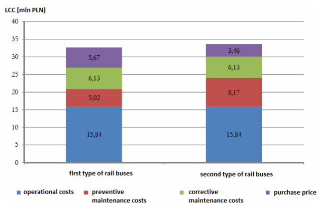
Figure 14. LCC structure for analysed types of rail buses [9]
