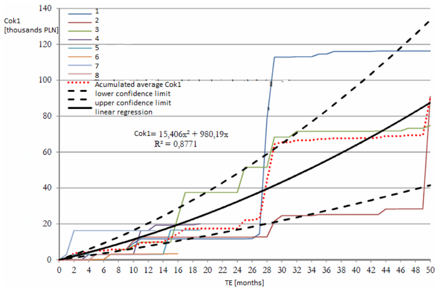
Figure 12. Corrective maintenance costs of analysed rail buses (failures group 1) [9]
