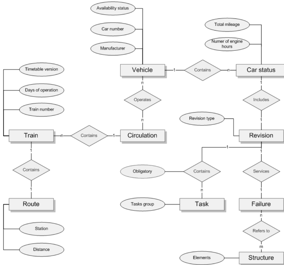
Figure 2. The model of railcar operation process shown as an entity-relationship-diagram [2]
