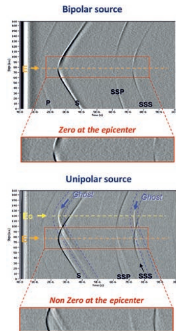
Fig. 8. Horizontal In-plane B-scans for a bipolar source and for a unipolar source after transmission through a 7.9 mm thick aluminum plate.
