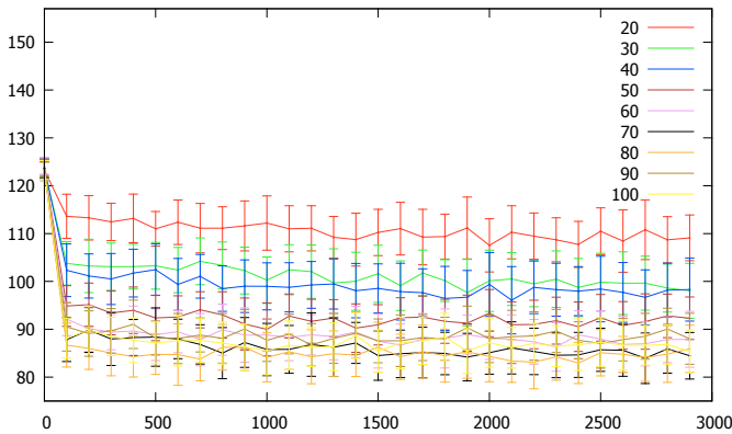
Figure 5. Influence of agent exchange energy on EMAS agent count agentCount(step) .
