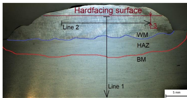
Fig. 1. Hardness measuring lines
