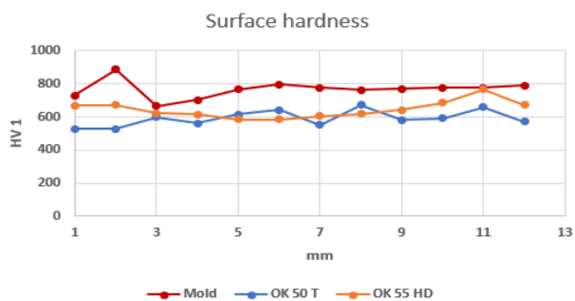
Fig. 4. Surface hardness
