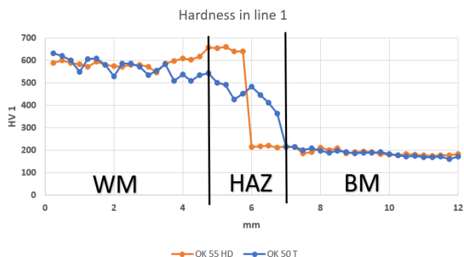
Fig. 5. Hardness profile
