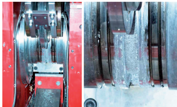
Fig. 5. Clamping element for the pre-compaction of chips in the groove of the extrusion wheel
