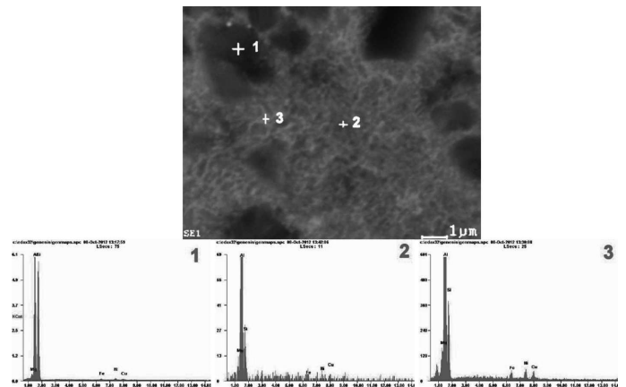
Fig. 11. Microstructure of the AlSi30 alloy rod consolidated by CRE and chemical analysis of the precipitates
