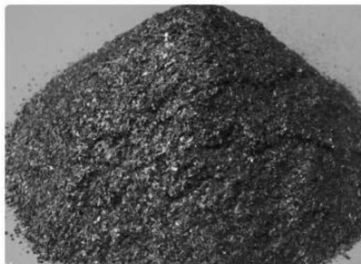
Fig. 3. Ribbon “chopped” into flakes in a cutting mill
