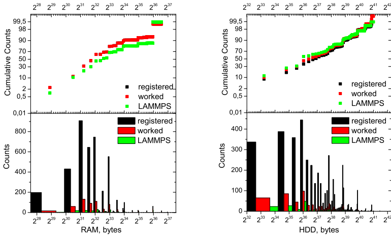
Figure 4. Distribution of the RAM sizes (left) and HDD sizes (right) for the registered hosts (black), the worked hosts (red), and the hosts used for LAMMPS-application (green).
