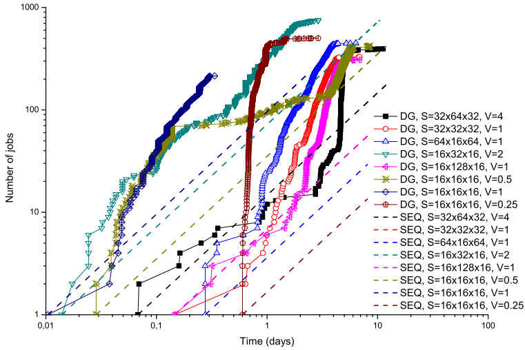
Figure 5. The number of calculated jobs as a function of time in the parallel distributed (DG) mode (symbols) and sequential (SEQ) mode (dash lines). The different types of jobs are denoted by different symbols and dash lines in the legend. S means the sizes of the simulated nanocrystal (in the lattice spacings), and V means the strain rate (in spacings per second).
