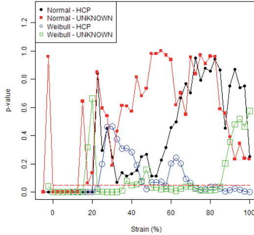
Figure 10. Kolmogorov-Smirnov test for distributions of defect concentrations: SFs (HCP), atom-vacancy states (UNK).
