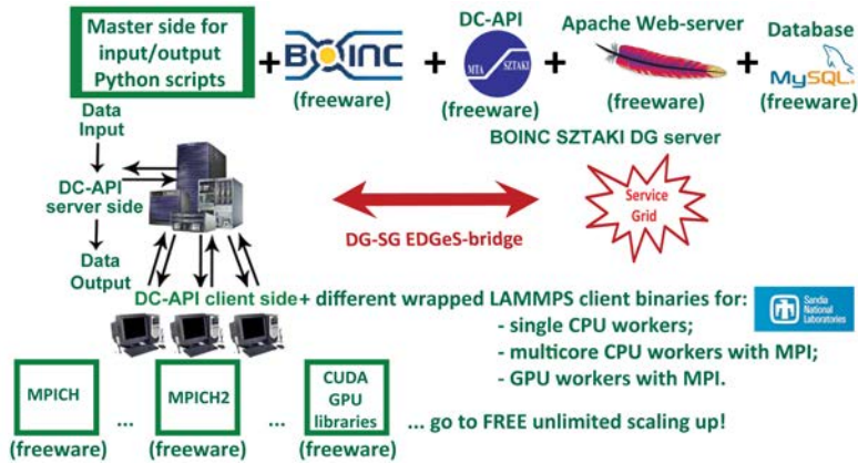
Figure 1. The general scheme of porting LAMMPSoverDCI application to DG-SG DCI for massive MD simulations with job distribution by SZTAKI DG approach [21].
