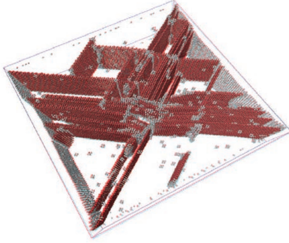
Figure 8. Tension of Al nanocrystal, strain \varepsilon = 7\% , orientation \langle 011 \rangle \{011\} . (It is anaglyph stereo figure, please, see explanations in the text.)
