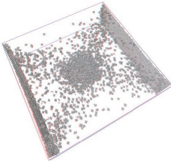
Figure 7. Tension of Al nanocrystal, strain \varepsilon = 7\% , orientation \langle 010 \rangle \{010\} . (It is anaglyph stereo figure, please, see explanations in the text.)
