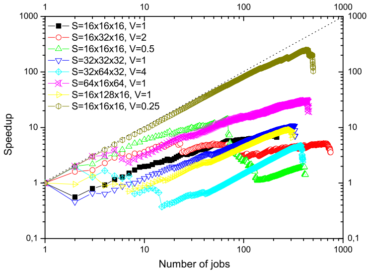
Figure 6. The effective speedup (the ratio of the total runtime in sequential and parallel distributed modes) for each type of job as a function of the jobs calculated in the parallel distributed (DG) mode (symbols) in comparison with the theoretical maximum (dash line). The different types of jobs are denoted by different symbols in the legend. S means the sizes of the simulated nanocrystal (in the lattice spacings), and V means the strain rate (in spacings per second).
