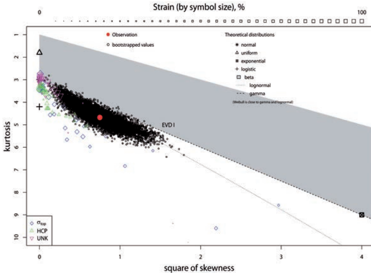
Figure 11. Pearson diagram for moment and bootstrapping analysis for: defect concentration distributions over the ensemble of nanocrystals for SFs (HCP), atom-vacancy states (UNK), and for the normal stress values \sigma_{top} at the atomic planes near grips of the testing machine.
