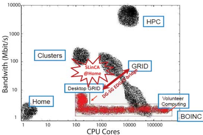
Figure 2. DG-SG DCI SLinCA@Home used for massive MD simulations in the context of the available HPC approaches (adaptation of the original figure by courtesy of Fermin Serrano).
