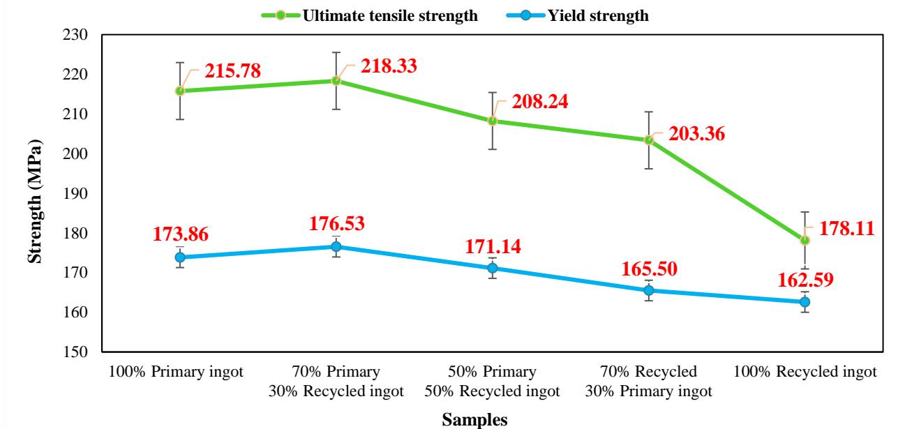
Fig. 7. Yield strength and ultimate tensile strength values of the samples
