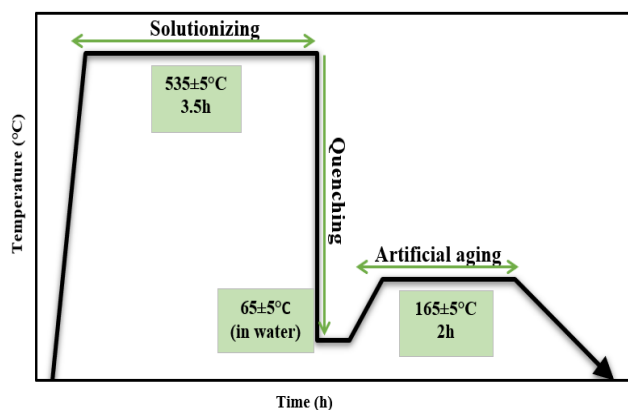
Fig. 2. T6 Heat treatment
