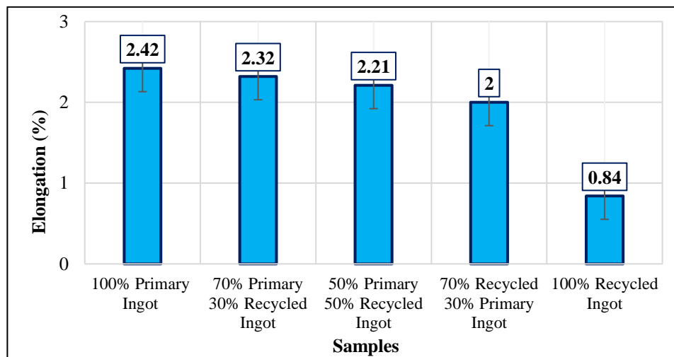
Fig. 8. Elongation values of the samples (%)
