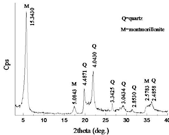
Fig. 1. X-ray diffraction diagram of purified bentonite
