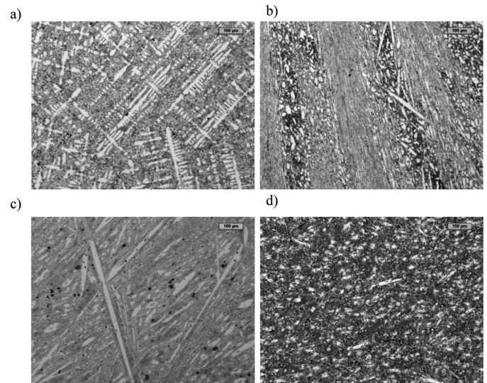
Fig. 2. Example of microstructures of castings made from high chromium cast iron: melt no. I/2 – (a), melt no. I/4 – (b), melt no. I/7 – (c), melt no. I/8 – (d)
