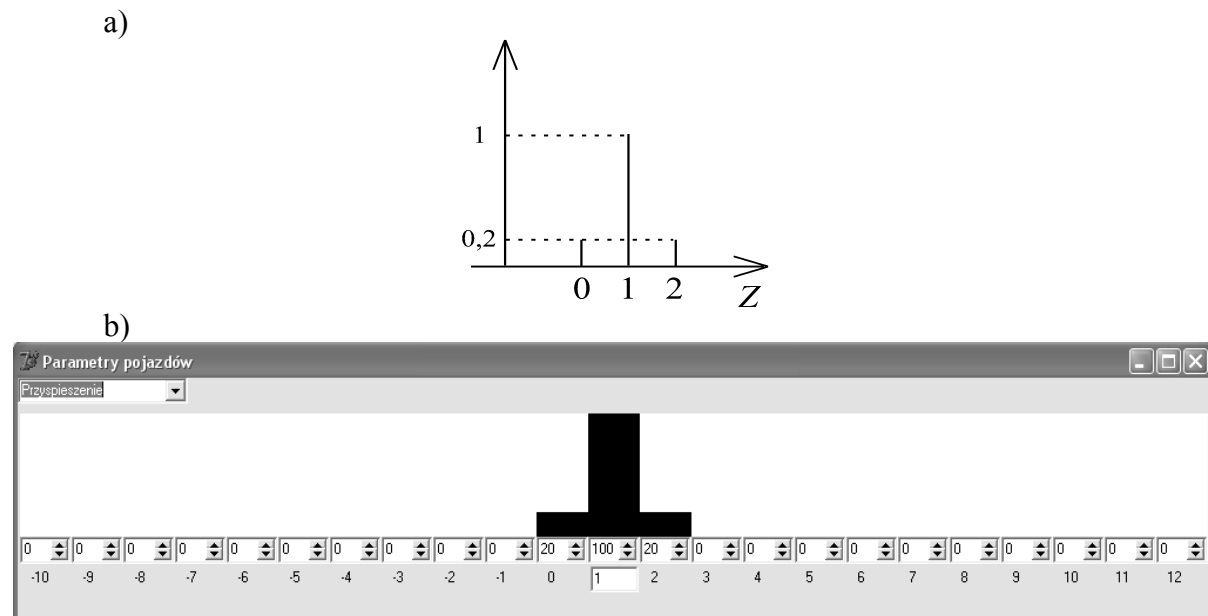
Fig. 2. a) Discrete membership function of fuzzy number that represents vehicle acceleration and b) the representation example for entering the data into the model
