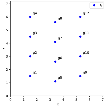
Fig. 2. Scenario G1 – a 3x4 recessed luminaire grid.
