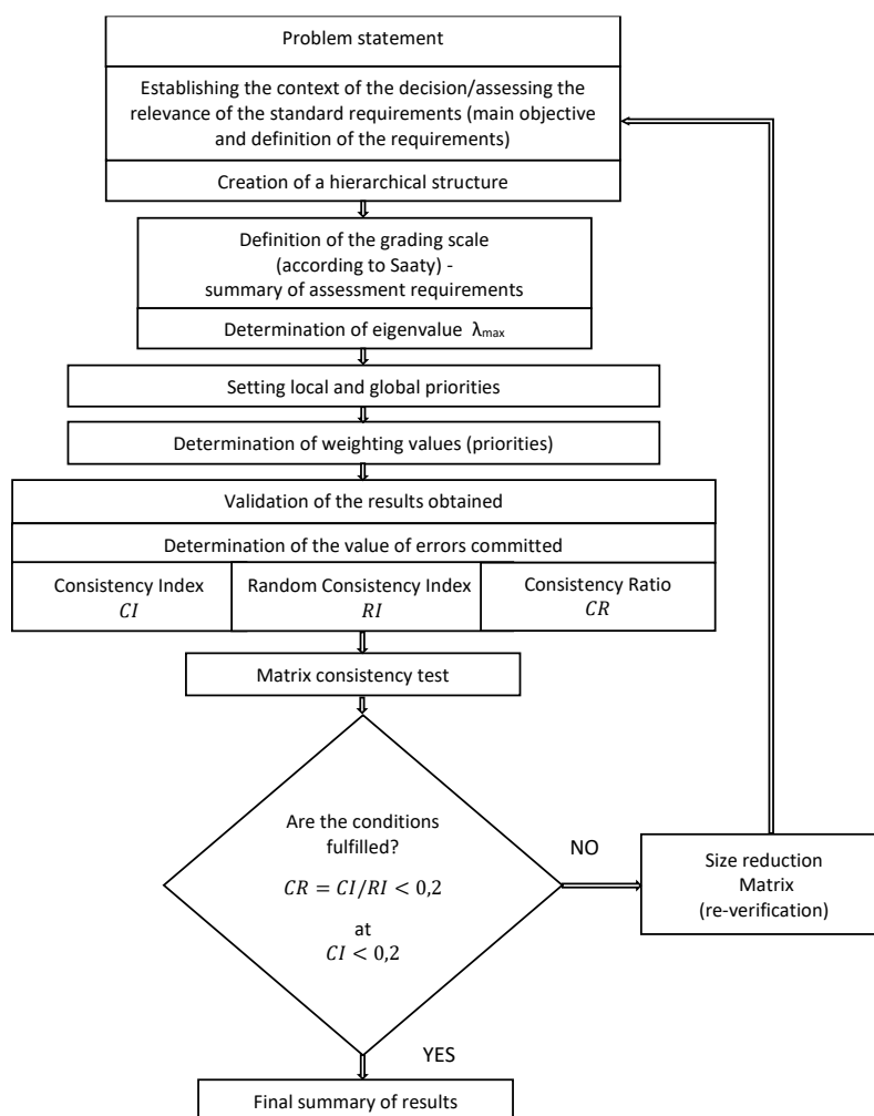
Fig. 1. Saaty method algorithm used to determine the weights
