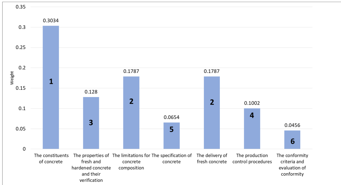
Fig. 2. Prioritisation of the standard requirements formulated in EN 206 based on the weights derived from the AHP analysis
