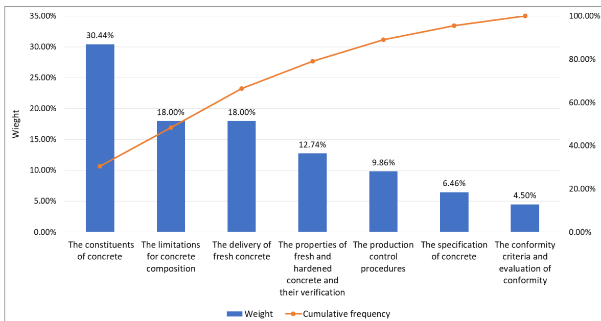
Fig. 3. Pareto chart based on the weights obtained from the AHP analysis for the standard requirements formulated in EN 206
