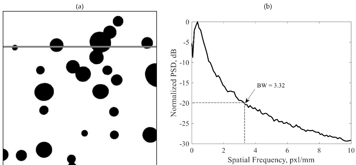
Fig. 4. (a) Example of binary image, and (b) normalized power spectral density and bandwidth estimation (Vinnett et al., 2018)
