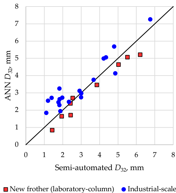
Fig. 9. Blind test: modelling performance using datasets with different characteristics to the training datasets. The red squares represent the results obtained using laboratory-scale data in a flotation column operated with a different frother (Flottec F120-20). The blue circles represent the results obtained from industrial-scale data. The continuous line corresponds to the ideal trend y = x
