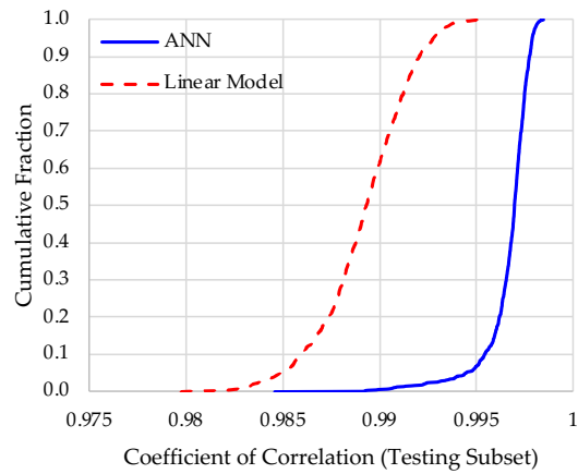
Fig. 6. Comparison of the cumulative distribution functions of the coefficient of correlation from the testing subsets: the ANN model versus the linear model proposed by Vinnett, Cornejo, et al. (2022)
