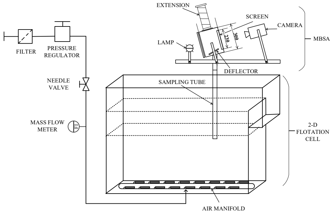
Fig. 2. Two-dimensional flotation cell and installation of the McGill bubble size analyser (Vinnett, Cornejo, et al., 2022)
