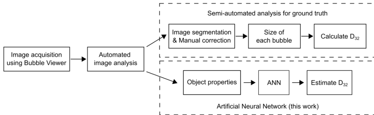
Fig. 1. Diagram of the data flow and estimation methodology used in this work. The semi-automated system was used to obtain the ground truth for D_{32} . An artificial neural network was trained to estimate the D_{32} based on the object properties obtained from an automated image analysis without segmentation.
