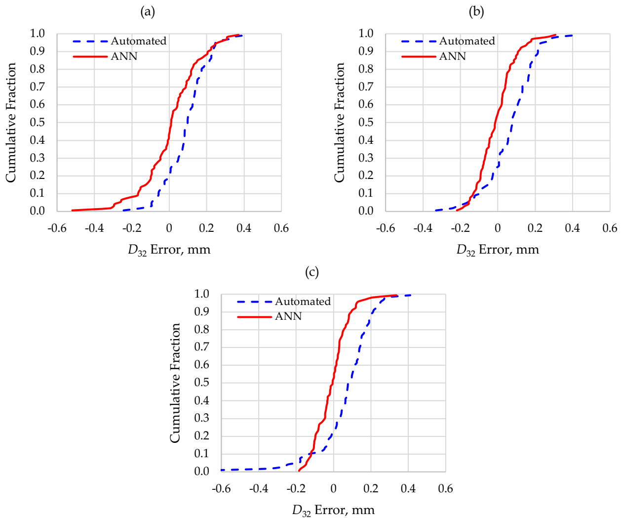
Fig. 8. Cumulative distribution functions of the D_{32} errors from the automated image processing and the ANN estimations. Experimental conditions that led to the (a) 2.5, (b) 50, and (c) 97.5 percentiles for correlation coefficient in the testing subsets
