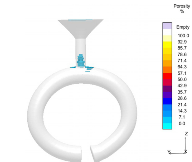
Fig. 21. Cast porosity using main sprue with dimensions matching radioscopic picture for artifact inv. no. 14/78 after 58 seconds from crystallization onset, mold heated to 600°C
