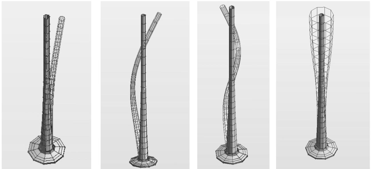
Fig. 3. Subsequent characters form of vibrations (displacements of chimney) as a function of frequency of vibration: form of vibration 1 (a), form of vibration 3 (b), form of vibration 6 (c), form of vibration 10 (d)
