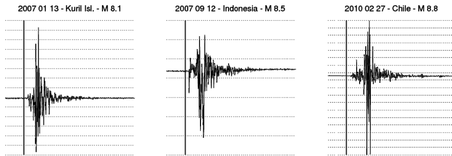
Fig. 3. Earthquakes in observations (every window is 7 h width, y grid is 1 mGal, vertical bar represents start of the Earthquake).
