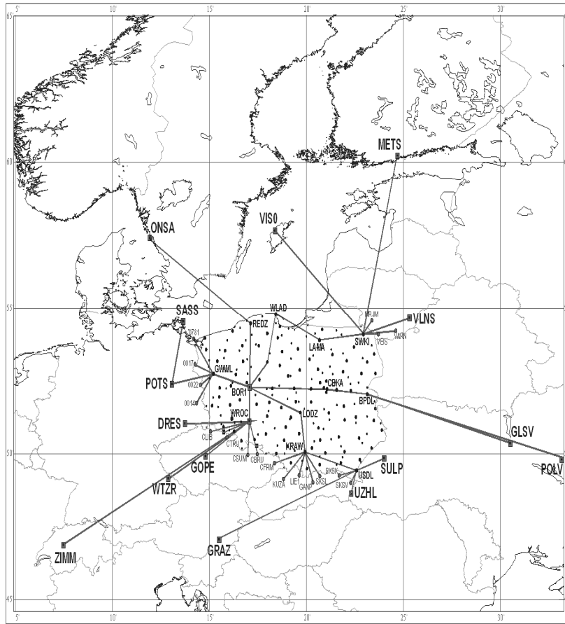
Fig. 3. EPN reference stations and connection vectors.
