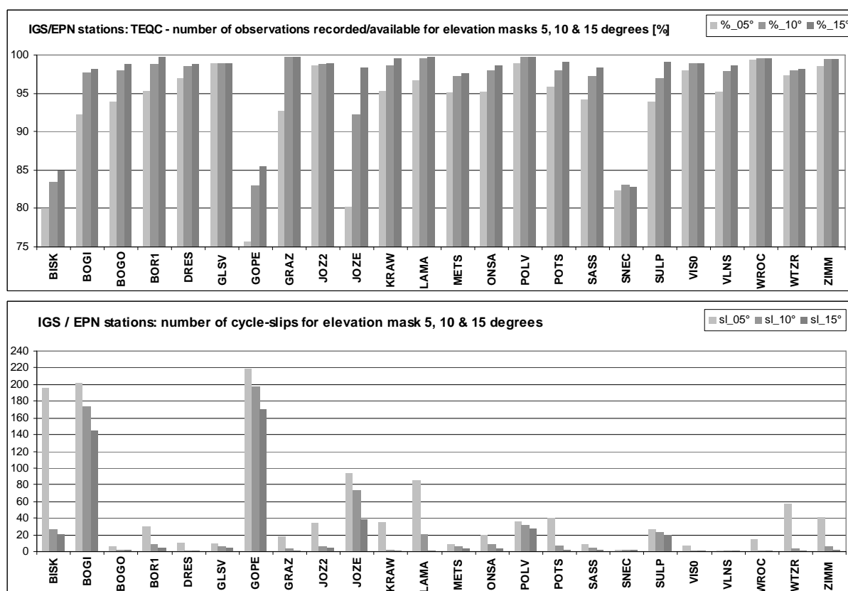
Fig. 2. Data analysis for EPN/IGS stations from TEQC program.
