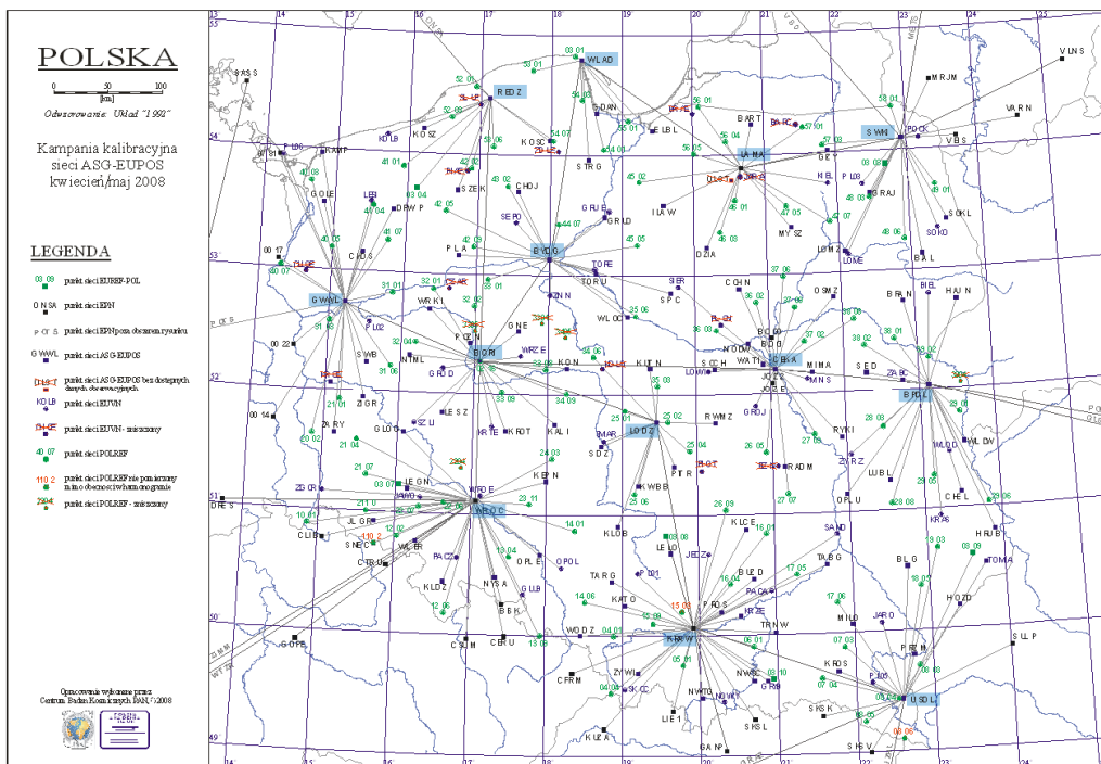
Fig. 4. Vector definitions for calibration campaign network solutions.
