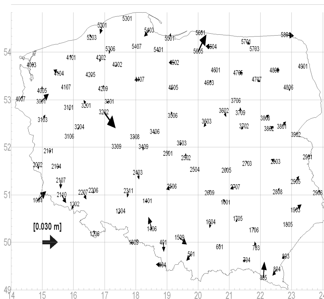
Fig. 5. Coordinate differences between POLREF and ASG-EUPOS network solutions (horizontal component).
