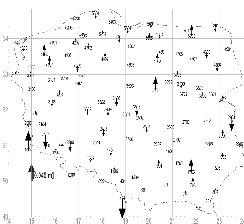
Fig. 6. Coordinate differences between POLREF and ASG-EUPOS network solutions (vertical component).
