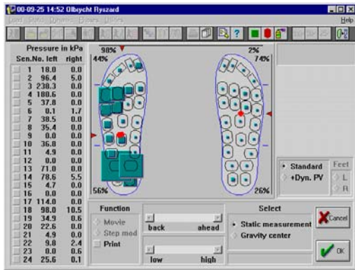
Fig. 7. Severe left hemiparesis; with a moved body weight
