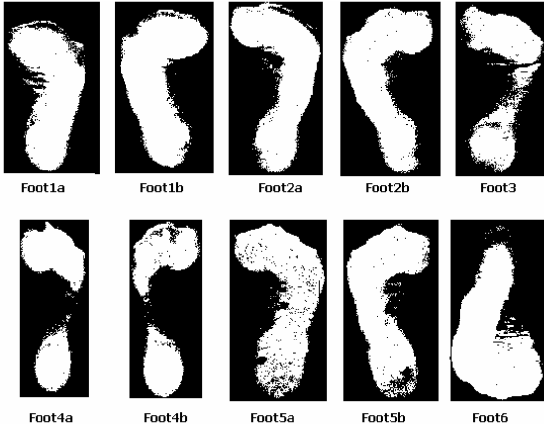
Fig. 6. The footprints examples used for analysis.
