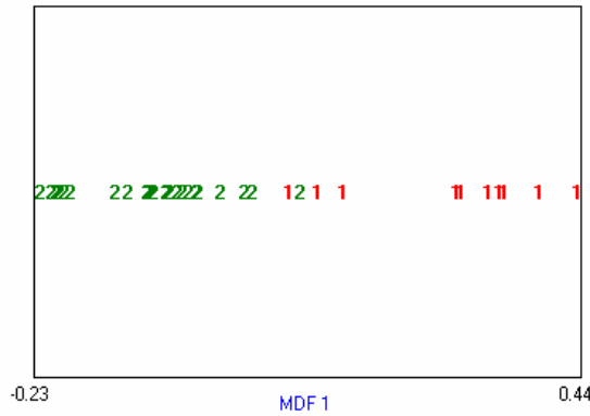
Fig. 8. LDA non-acceptable separation of cluster
