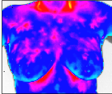
Fig. 3. Example of thermal image of healthy breast
