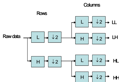
Fig. 1. Wavelet transformation of an image
