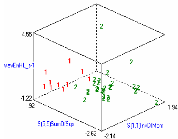
Fig. 7. Raw data analysis result
